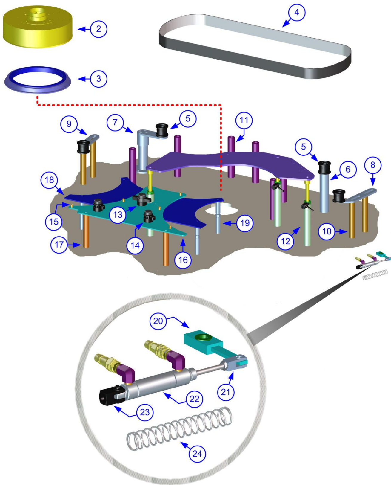
Figure 10, Table Assy
