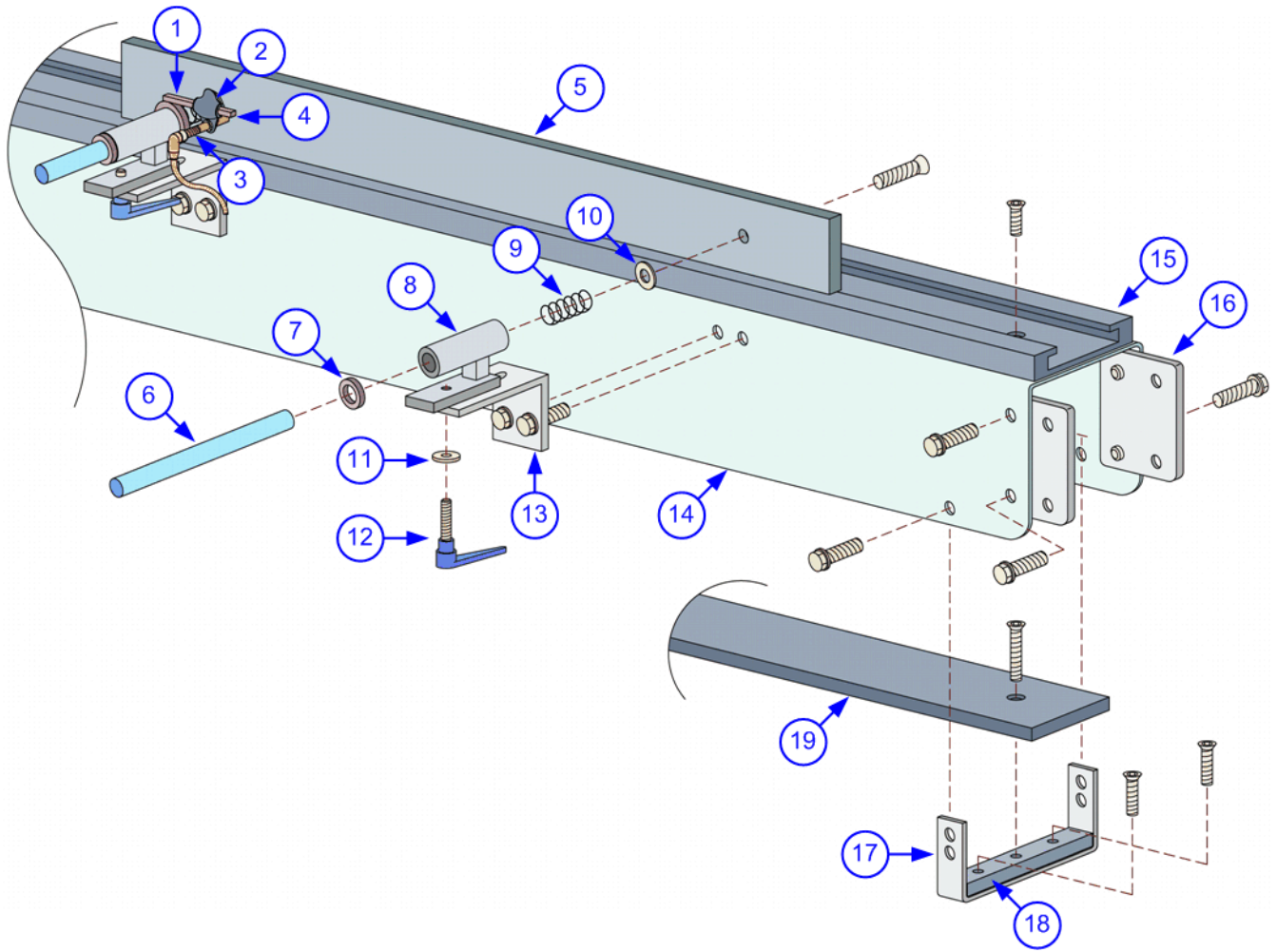
Figure 7, Conveyor Assembly
