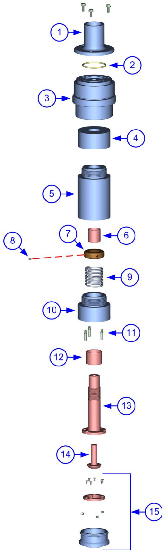
Figure 6, Chuck Assembly
