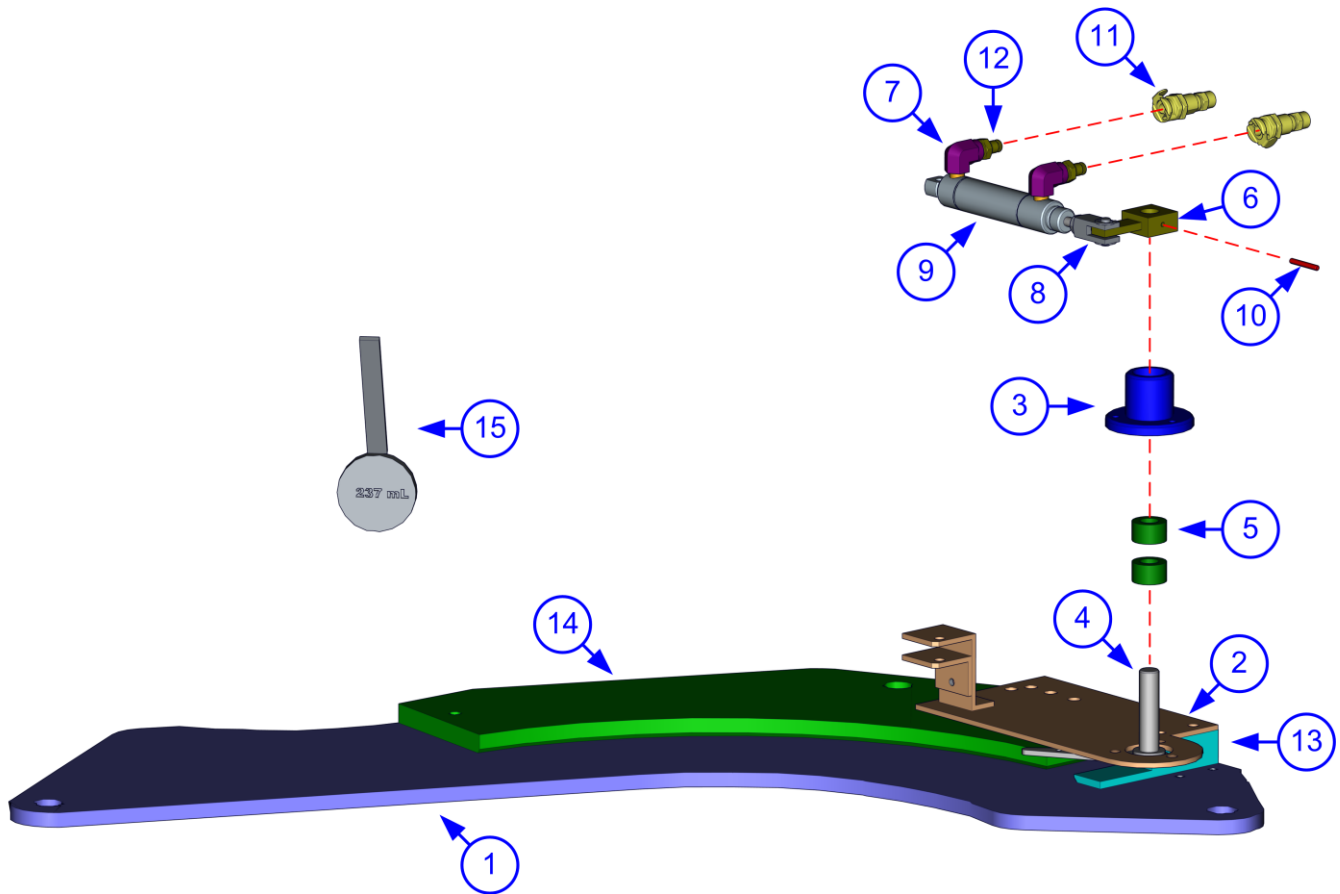
Figure 9, Cap Feed Assembly
