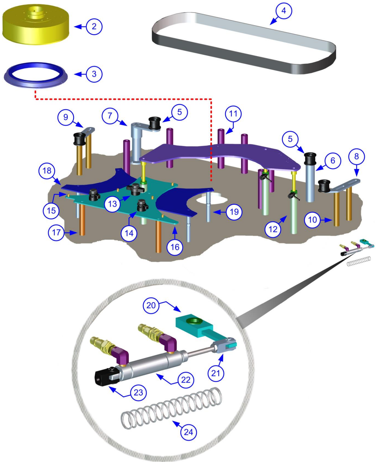
Figure 10, Table Assy
