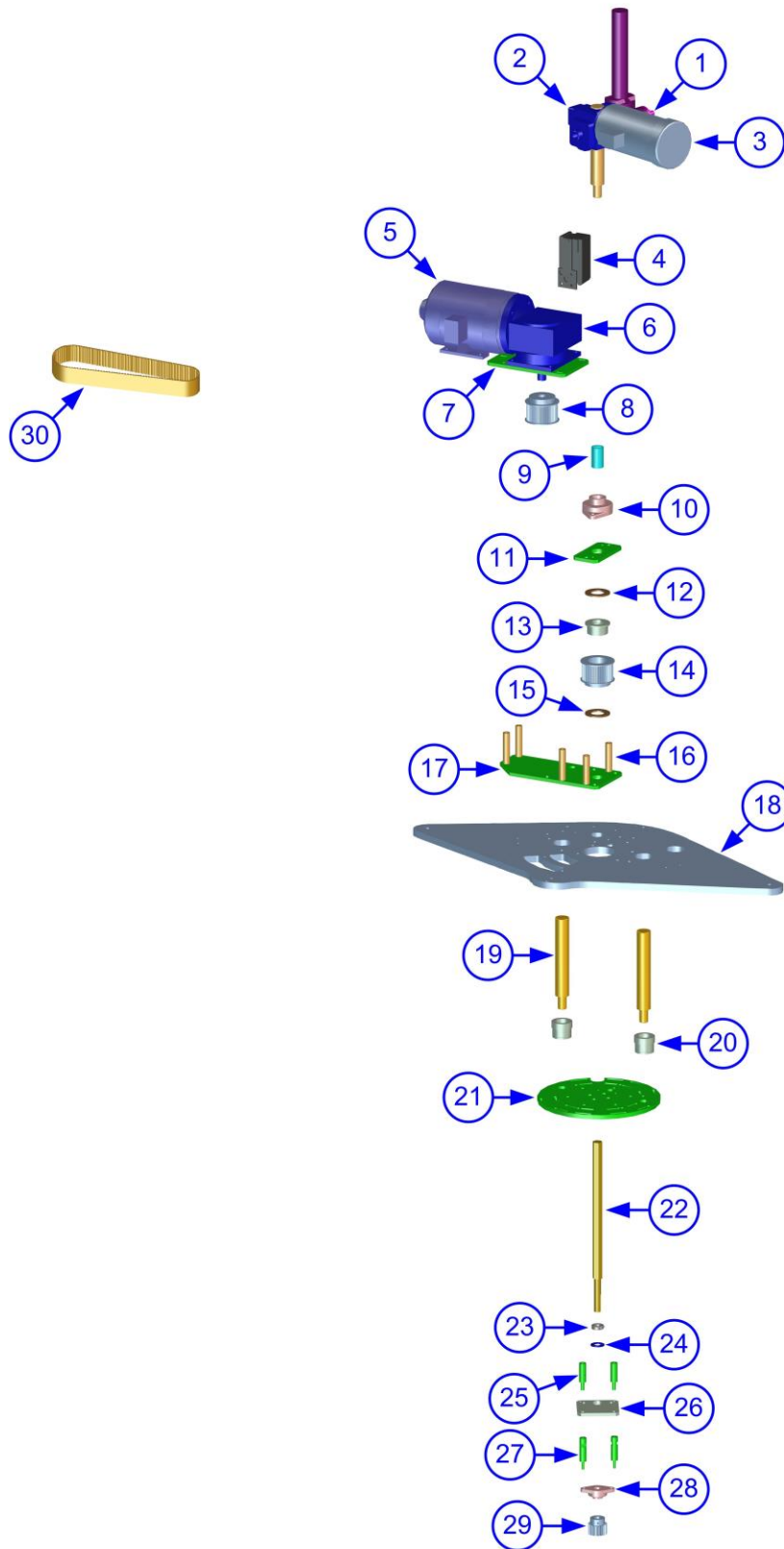
Figure 2, Capper Lift Assembly
