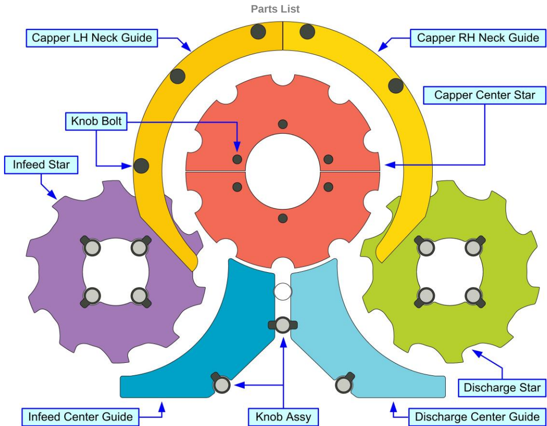
Figure 11, Attachments
