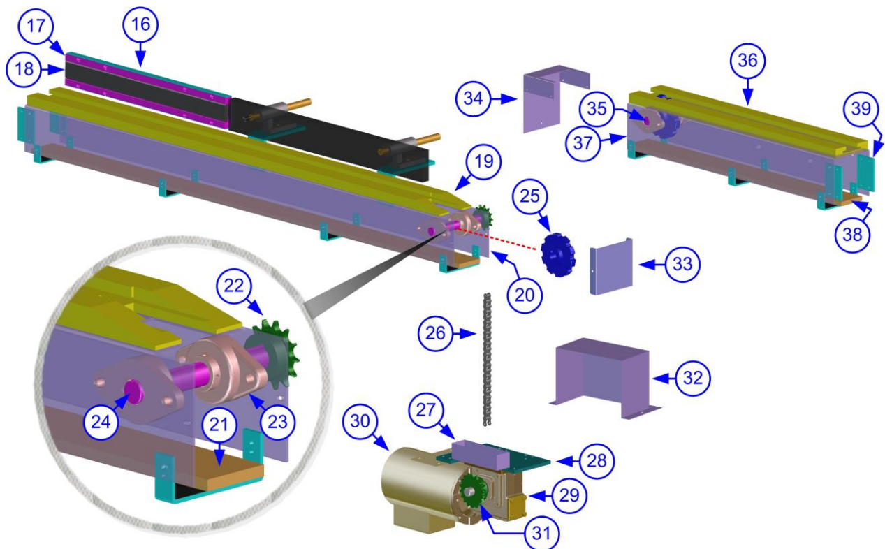
Figure 7b, Conveyor Assembly
