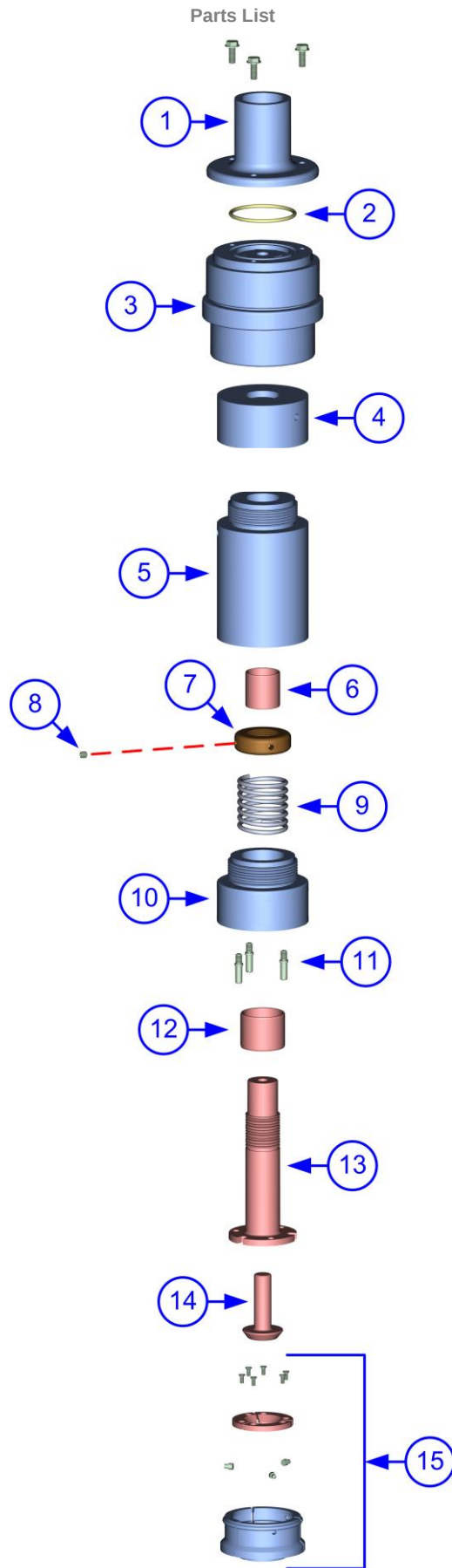
Figure 6, Chuck Assembly
