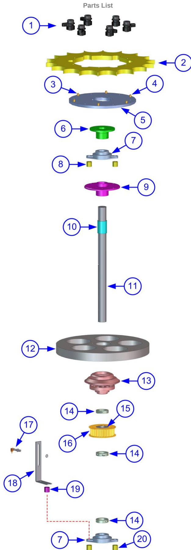
Figure 3, Infeed Star Shaft Assembly
