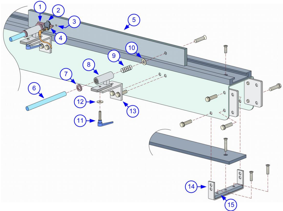
Figure 7a, Conveyor Assembly
