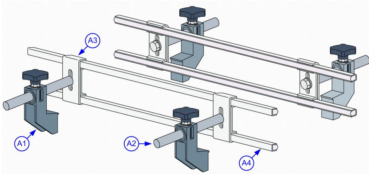
Figure 7c, Conveyor Assembly
