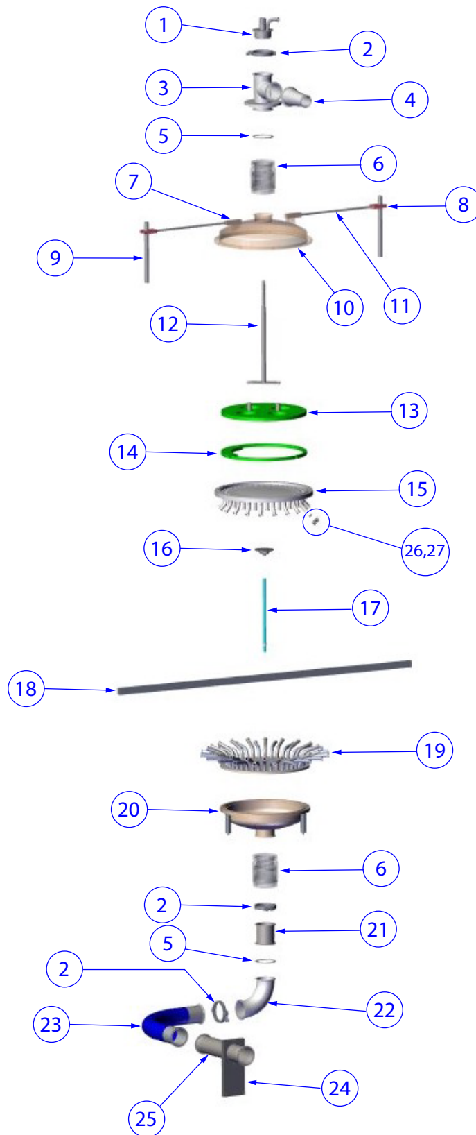
Figure 4-27: Filler Liquid System Assembly
