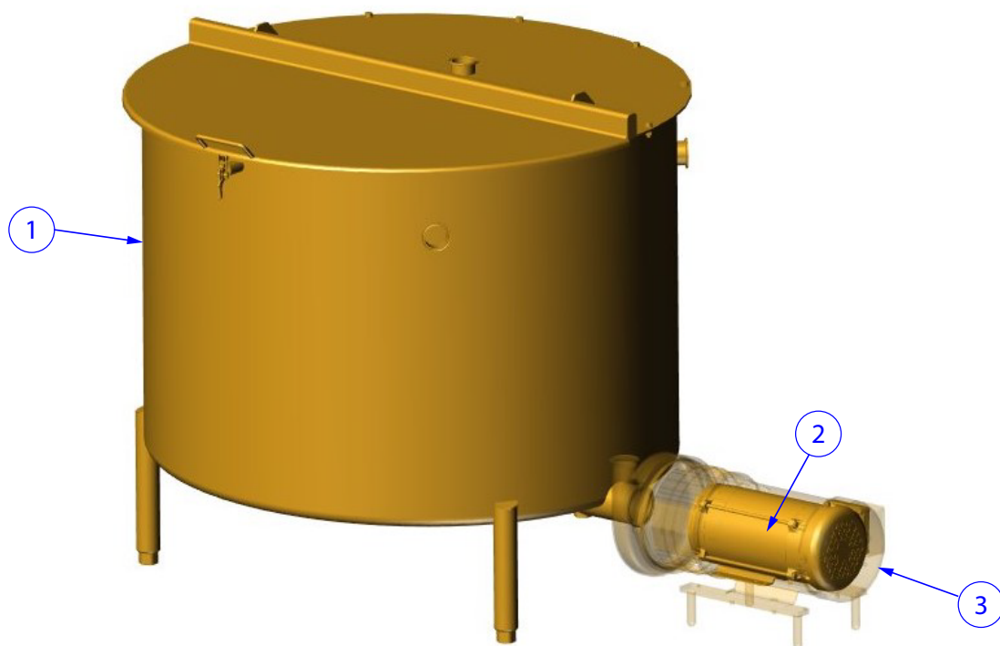
Figure 4-31: Production Tank-Pump/Motor Pressure System
