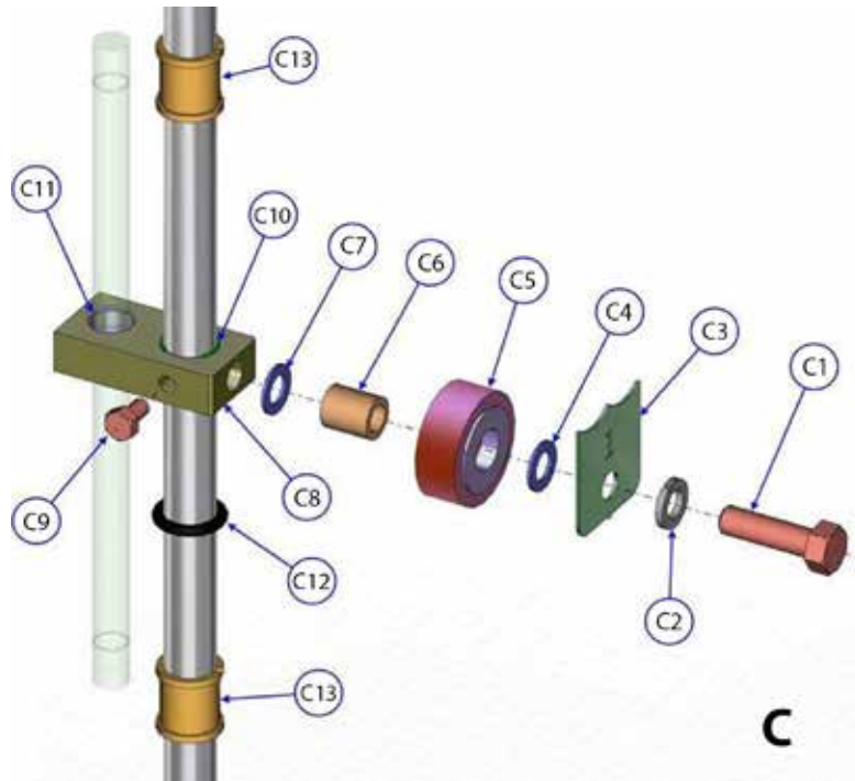
Figure 4-22: Filler Lift Roller Assembly
