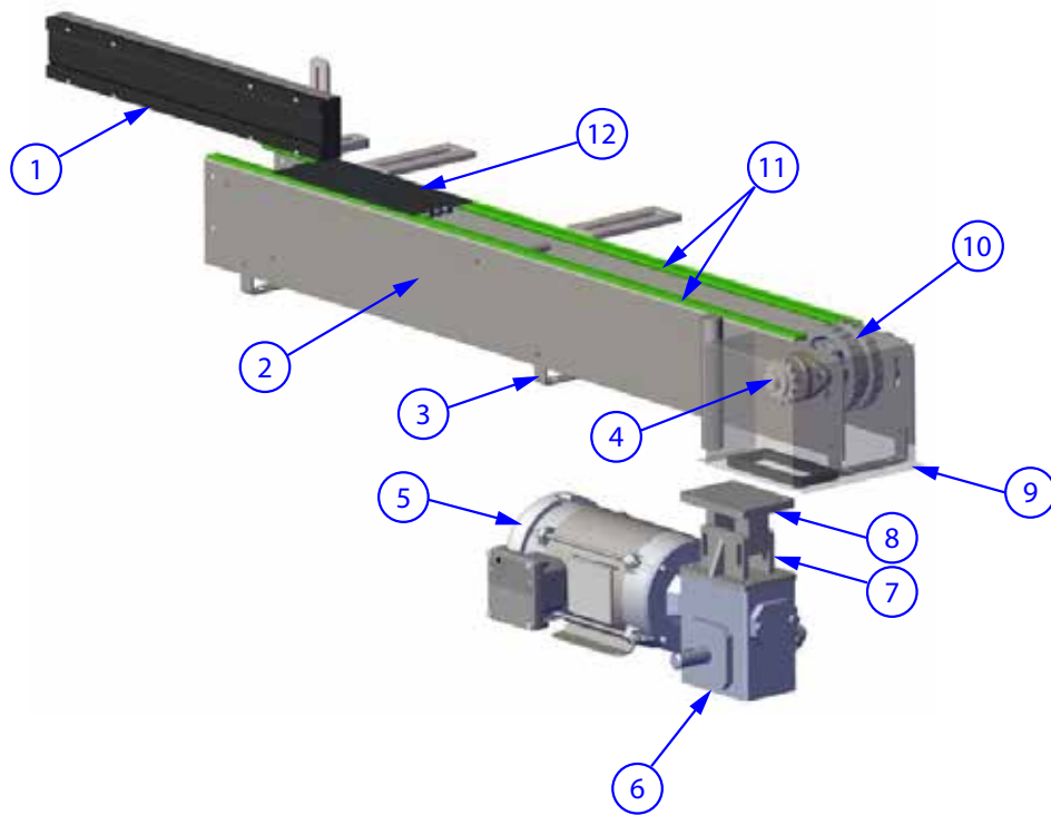
Figure 4-8: Conveyor Assembly (a)
