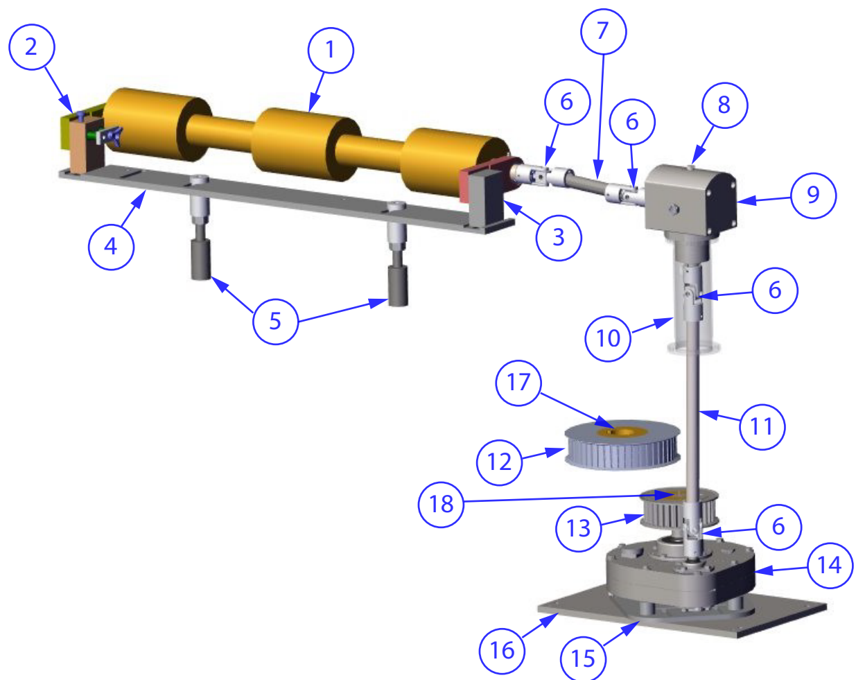
Figure 4-5: Worm Drive Assembly
