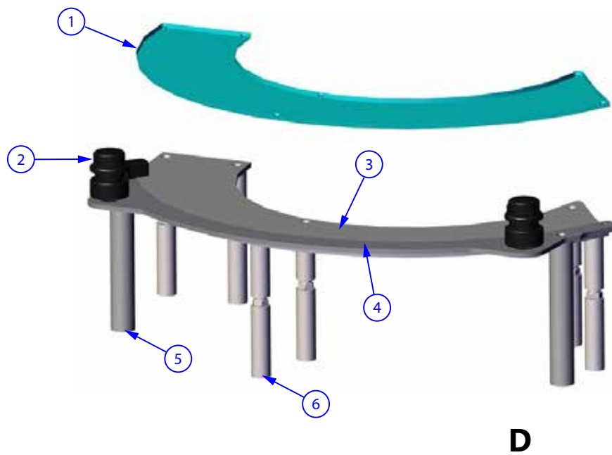
Figure 4-23: Filler Plates Assembly
