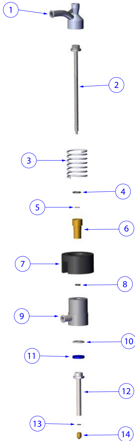
Figure 4-28: Filler Valve Assembly
