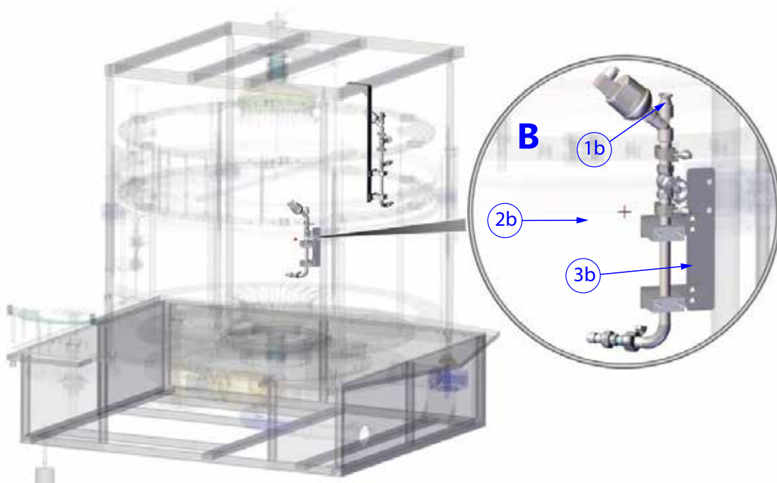
Figure 4-34: R.O. Wash System_b
