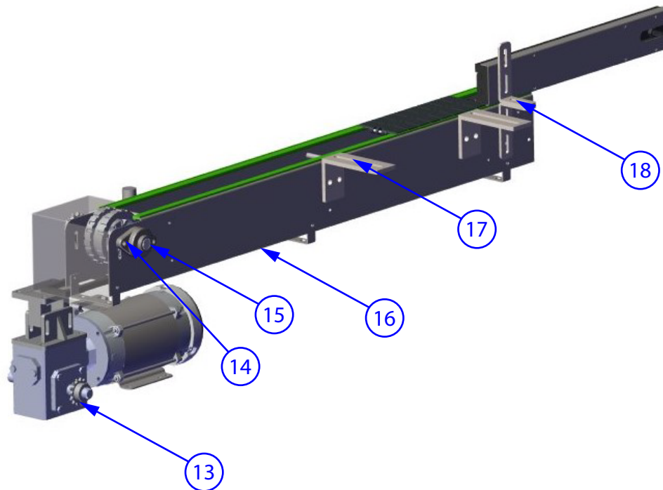
Figure 4-9: Conveyor Assembly (b)
