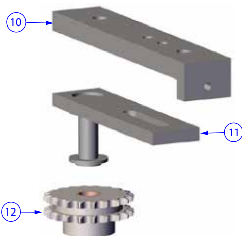
Figure 4-18: Idler Bracket Assembly
