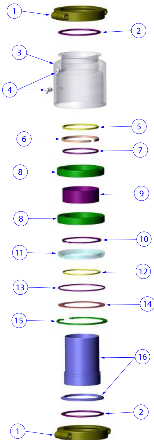
Figure 4-26: Filler Rotary Union Assembly
