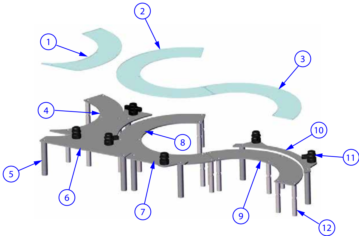
Figure 4-10: Rinser Plates
