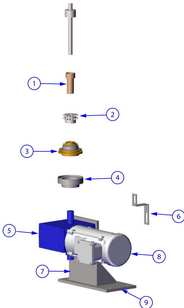
Figure 4-17: Filler Lift Assembly
