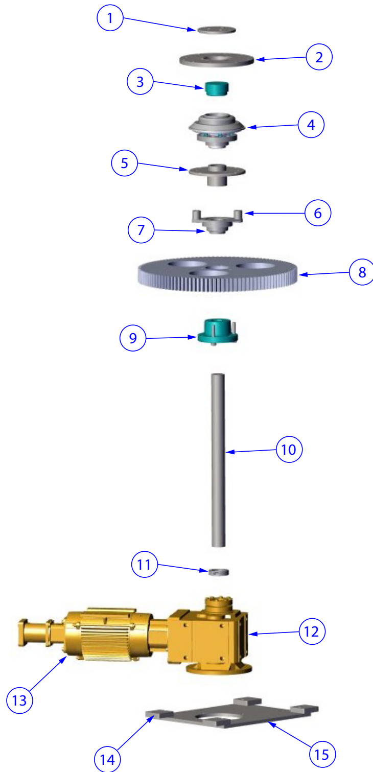
Figure 4-37: Capper Motor Drive Train Assembly
